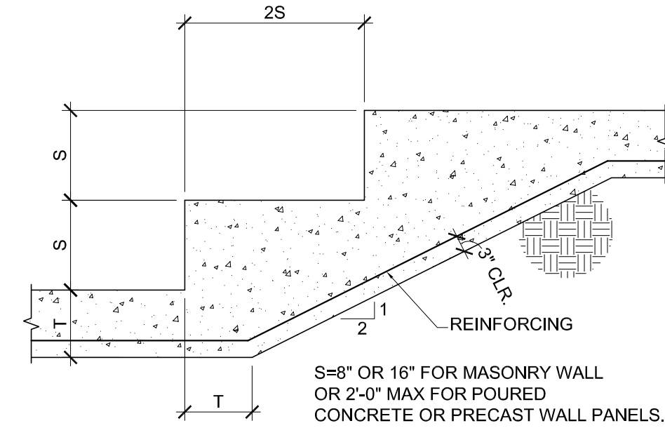
3 TYPICAL STEP FOOTING DETAIL SCALE: NO SCALE
