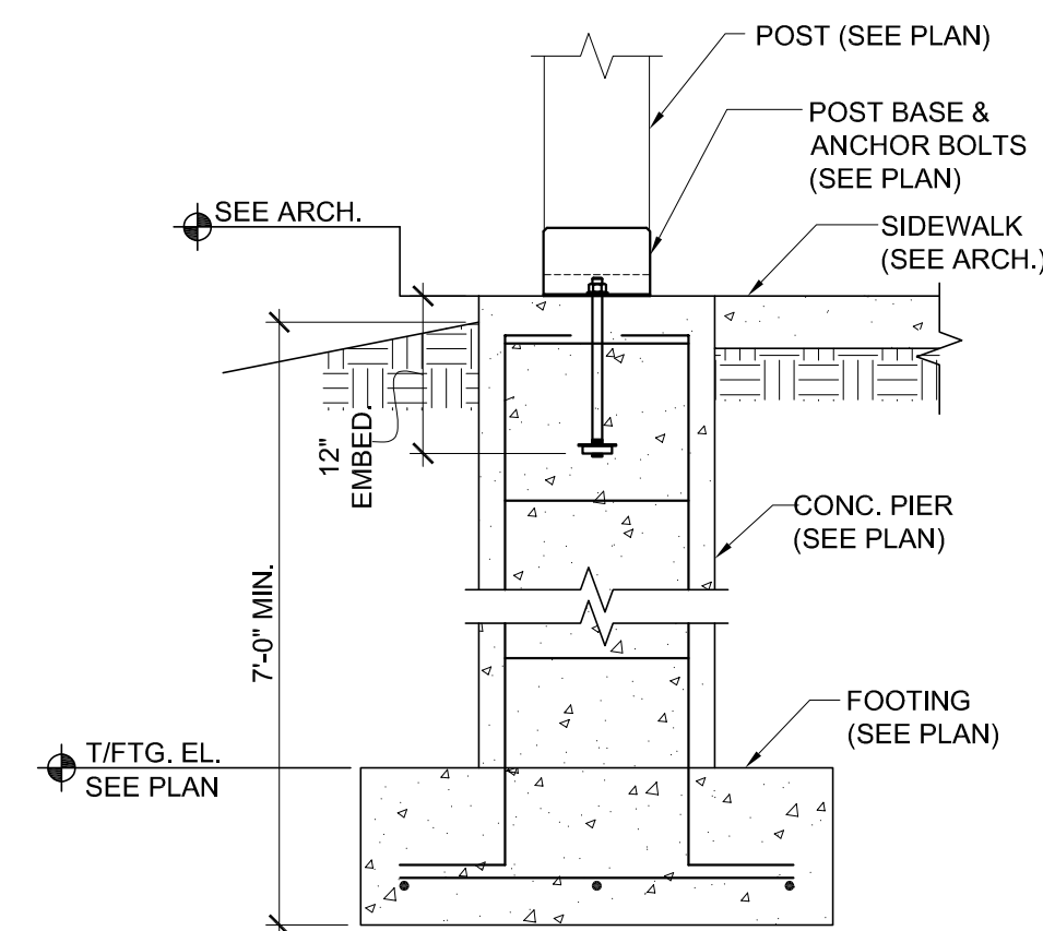
11 ENTRY POST DETAIL SCALE: NO SCALE
