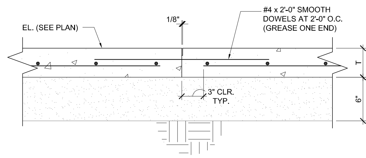
1 TYPICAL CONSTRUCTION JOINT DETAIL SCALE: NO SCALE
