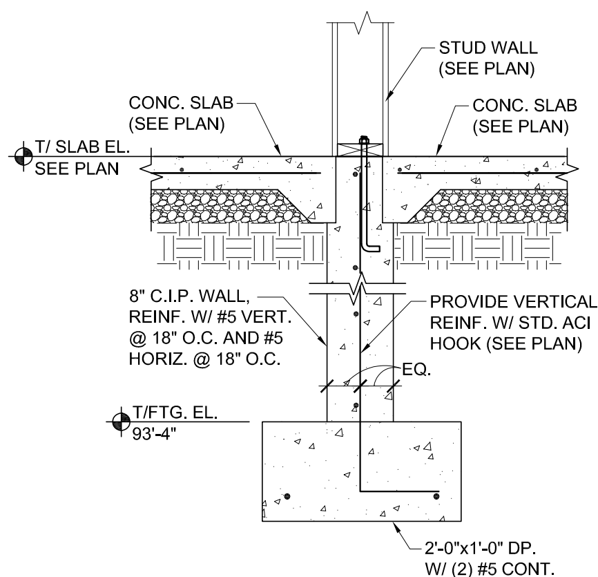
10 INTERIOR FTG. - ALT. FOR WINTER CONSTRUCTION SCALE: NO SCALE
