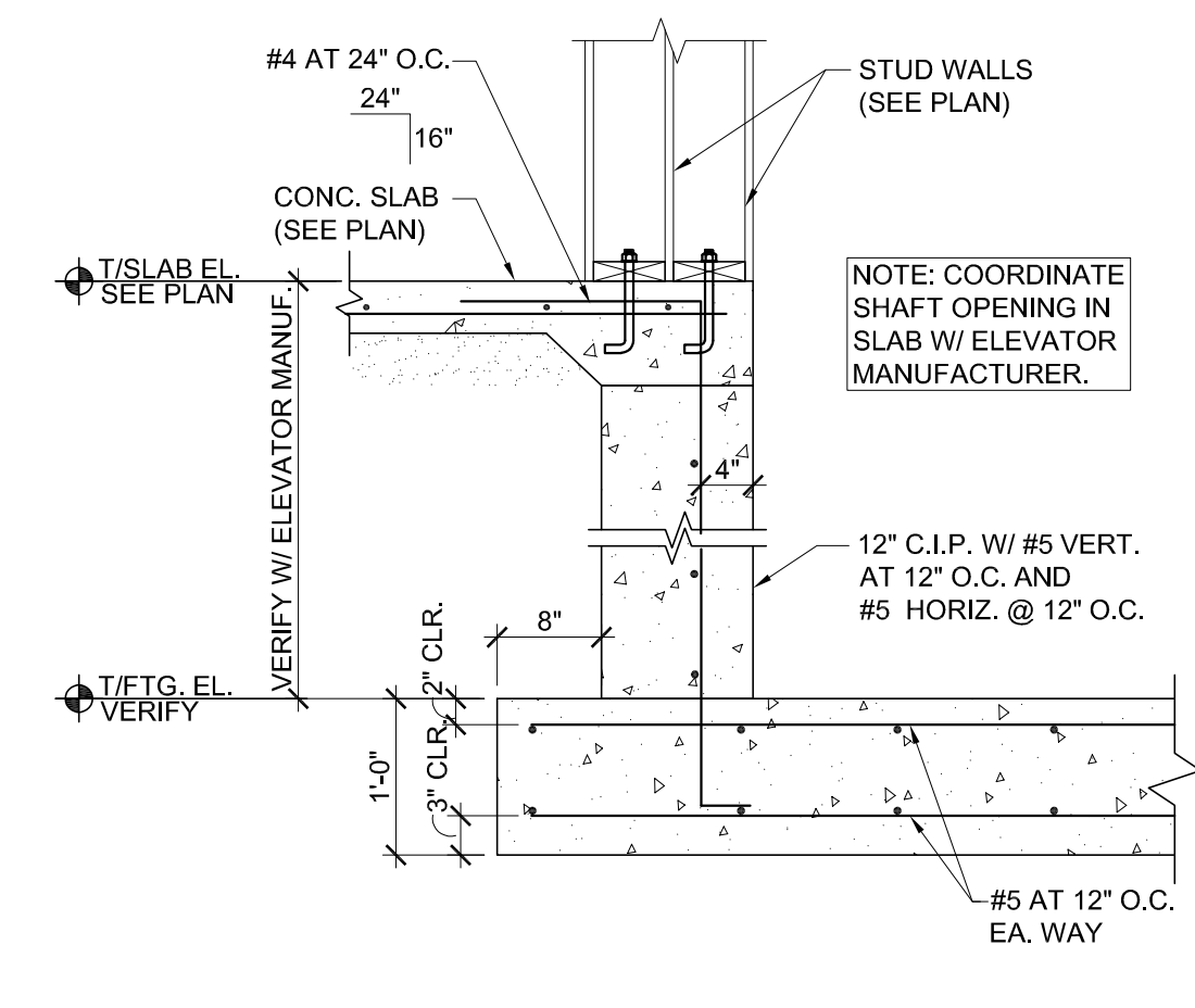
9 ELEVATOR PIT DETAIL SCALE: NO SCALE
