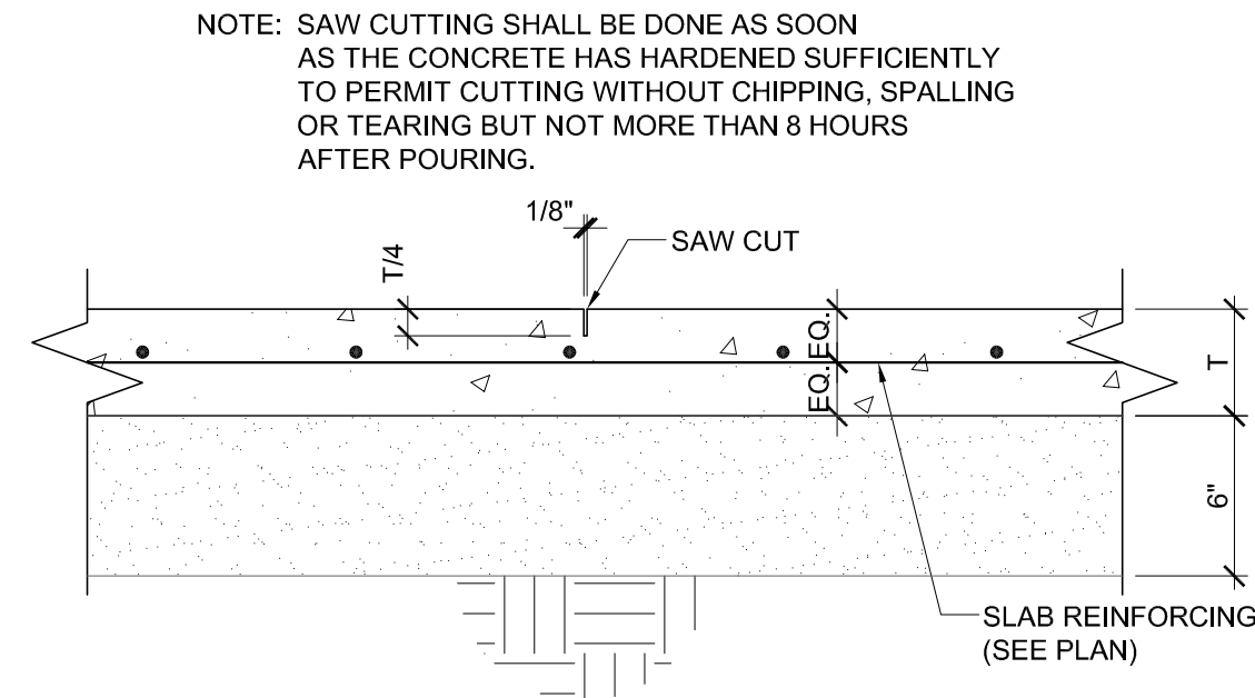
2 TYPICAL CONTROL JOINT DETAIL SCALE: NO SCALE
