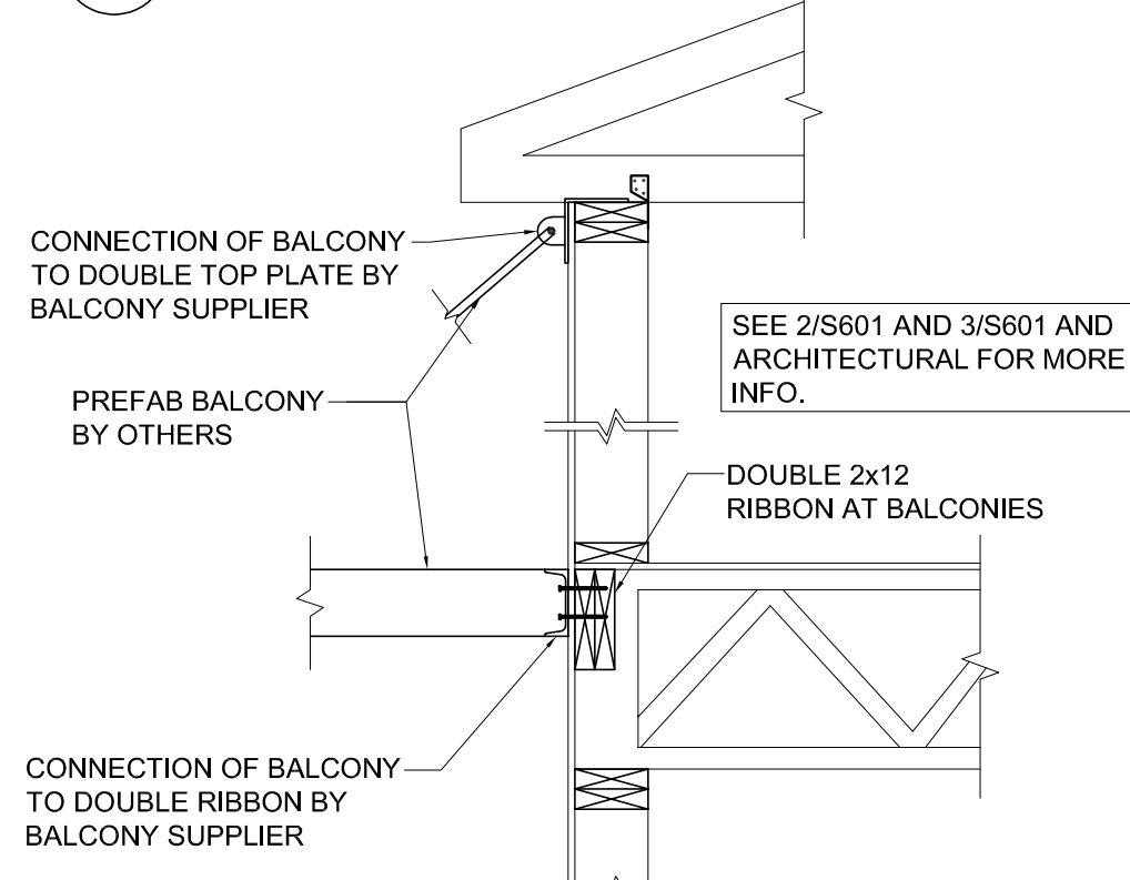
16 SECTION AT PRE-FAB BALCONIES SCALE: NO SCALE
