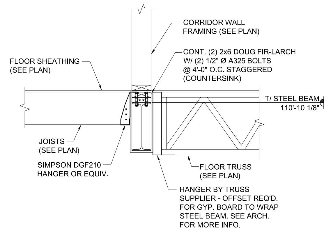
13 DETAIL AT STEEL BEAM SCALE: NO SCALE
