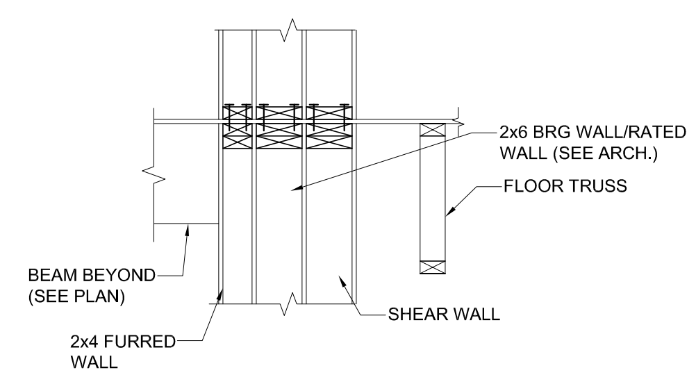
15 BEARING DETAIL @ FURRED WALL SCALE: NO SCALE
