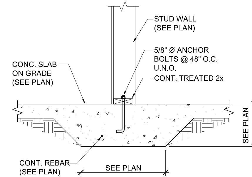
4 THICKENED SLAB FOOTING DETAIL SCALE: NO SCALE
