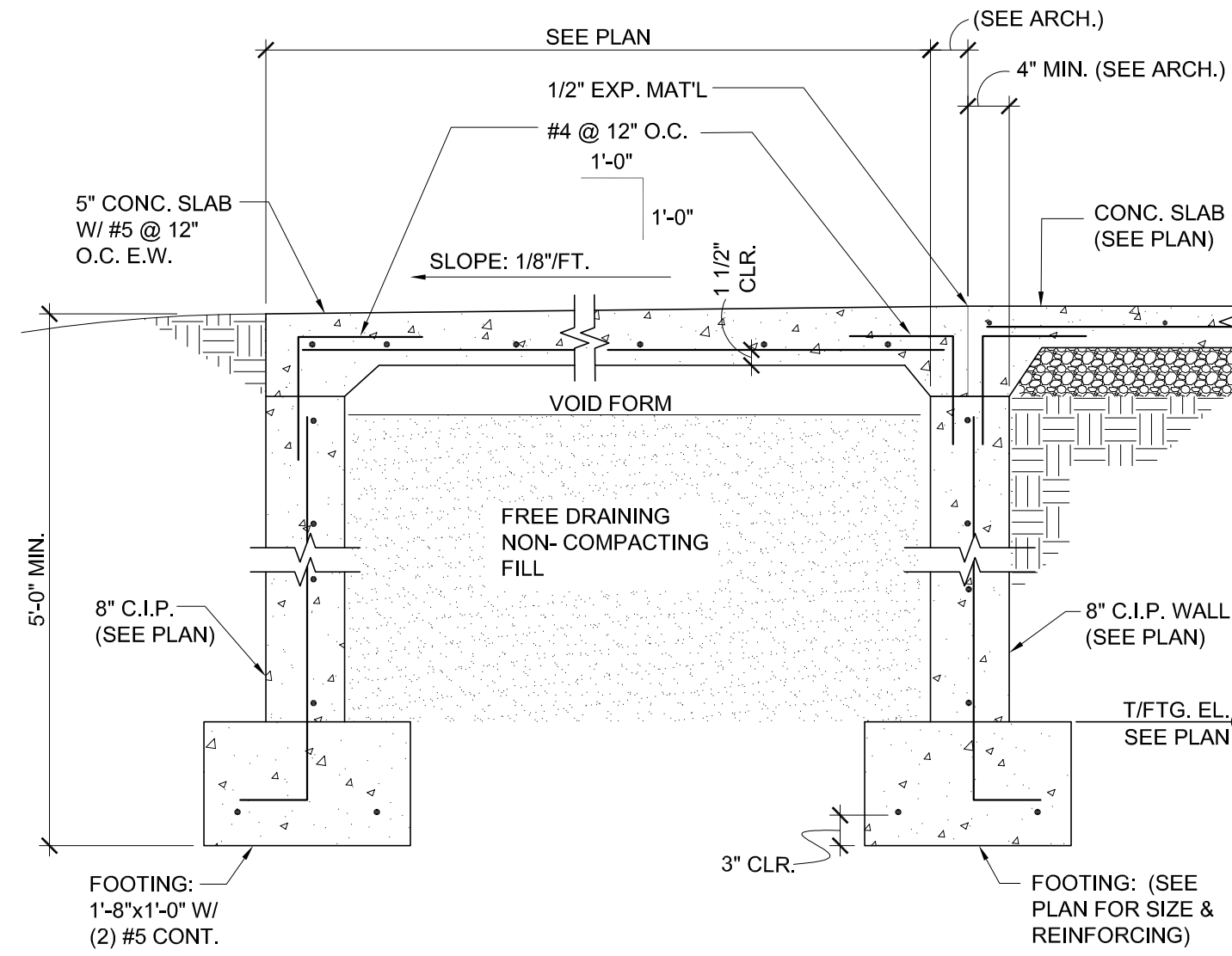
8 TYPICAL STOOP DETAIL SCALE: NO SCALE
