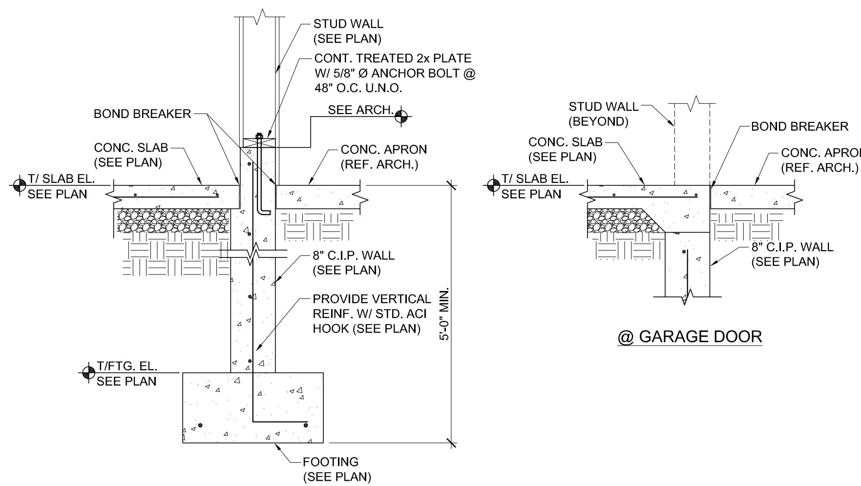
7 EXTERIOR WALL DETAIL @ GARAGE SCALE: NO SCALE
