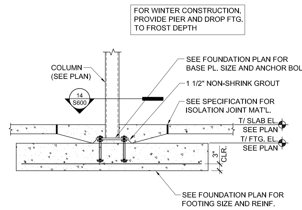
12 TYPICAL INTERIOR STEEL COL. FOOTING DETAIL SCALE: NO SCALE
