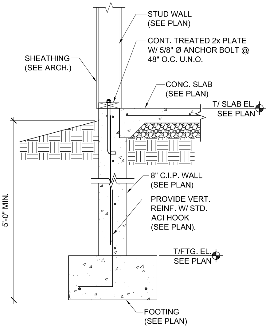
6 TYP. EXTERIOR WALL DETAIL SCALE: NO SCALE
