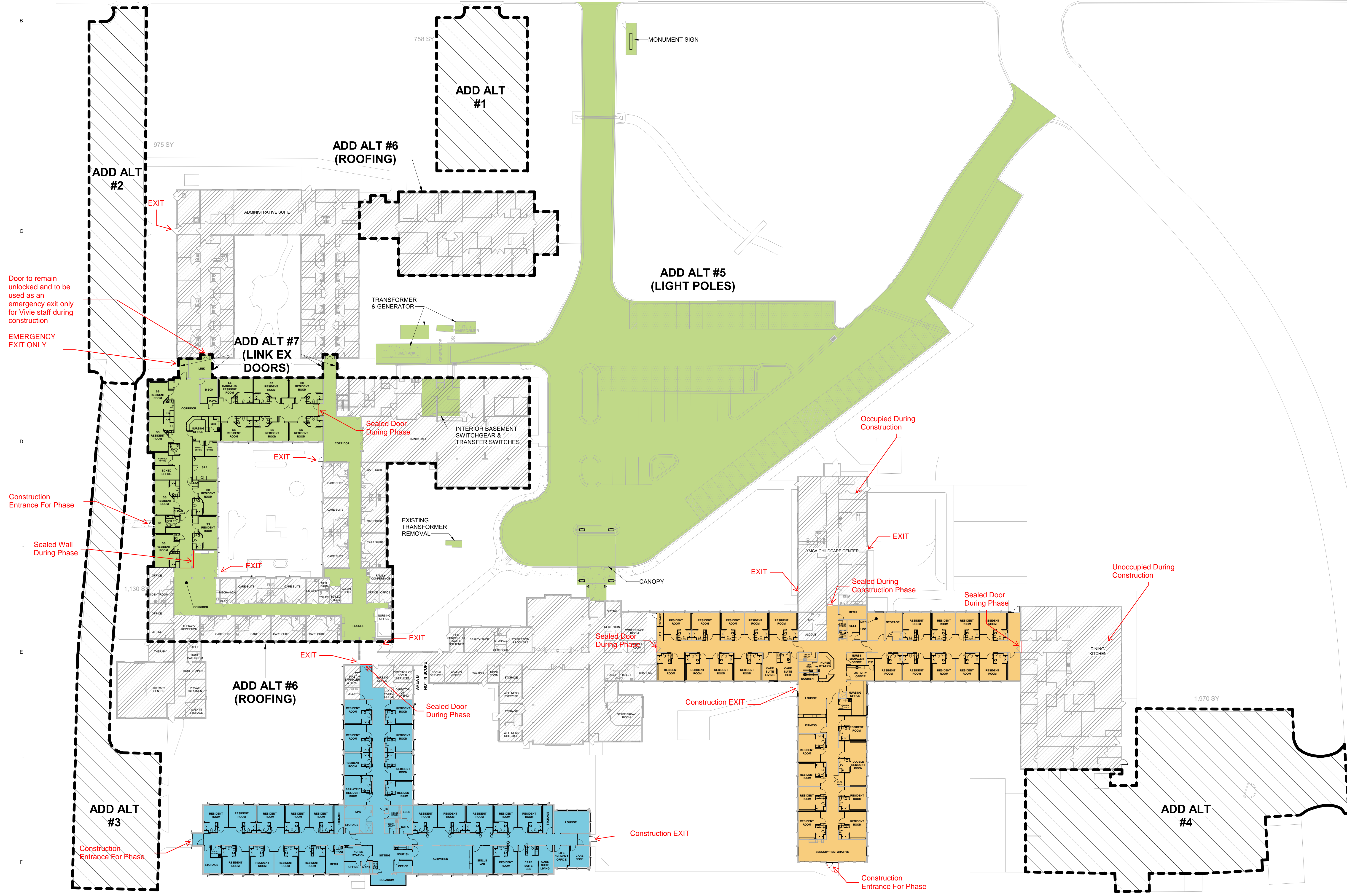
F1 OVERALL BUILDING PHASING PLAN 1" = 30'-0"
